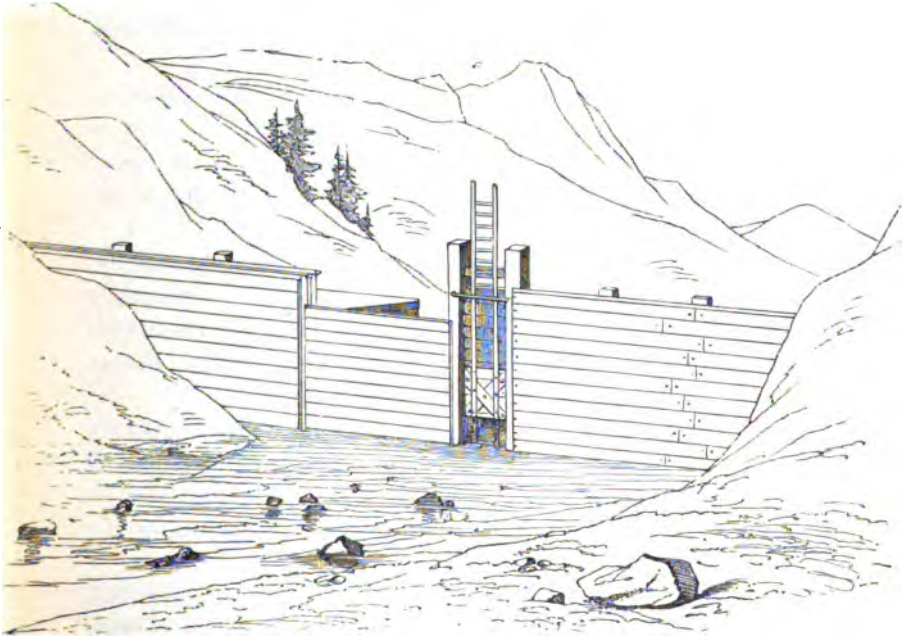
Fig. 232.—Wooden dam at Absdach (Black Forest).
